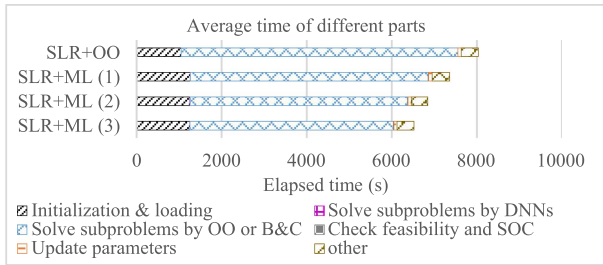
Fig. 9. Average elapsed time spent on various functions SLR+ML and SLR+OO for the Polish 2383-bus system.
